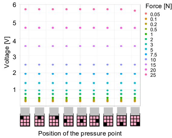
Fig. 7. The sensitivity of the strain gage force sensor to the pressure point. Finger position on the sensor is presented along the x -axis.
