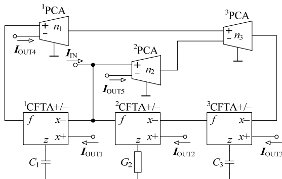
Fig. 4. Designed current-mode frequency filter.
