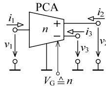
Fig. 2. Schematic symbol of PCA.
