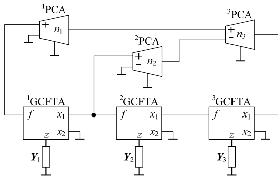
Fig. 3. Initial general autonomous circuit.
