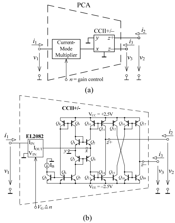
Fig. 6. (a) Block diagram of PCA element, (b) realization of the PCA using current multiplier EL2082 and second-generation current conveyor CCII+/-.
