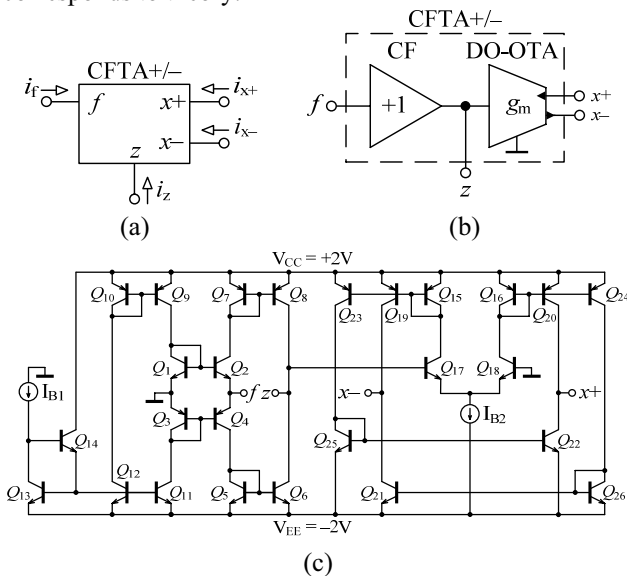
Fig. 5. (a) Schematic symbol, (b) block diagram, and (c) used bipolar implementation of CFTA+/- element.
